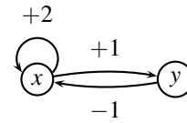
Fig. 1. GRN of mucus production in Pseudomonas aeruginosa . The gene x synthesizes a protein which activates the expression of gene y (when its concentration level exceeds the abstract threshold 1) and itself (when it exceeds 2) by binding the promoters. In turn, the protein of y inhibits the expression of x when its concentration level exceeds 1.
