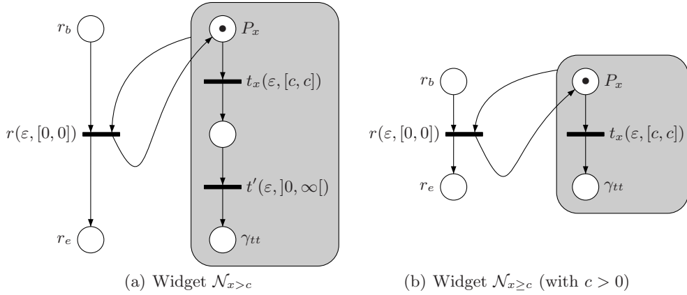
Fig. 2. Widgets for \mathcal{N}_{x>c} and \mathcal{N}_{x>=c}
