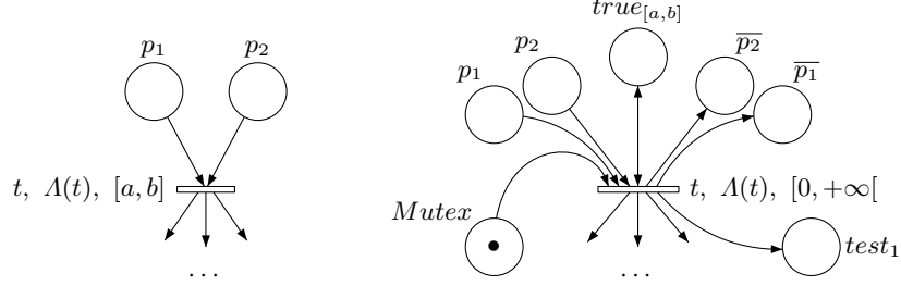
Fig. 7. From a transition in \mathcal{N} to its translation in \bar{\mathcal{N}}
